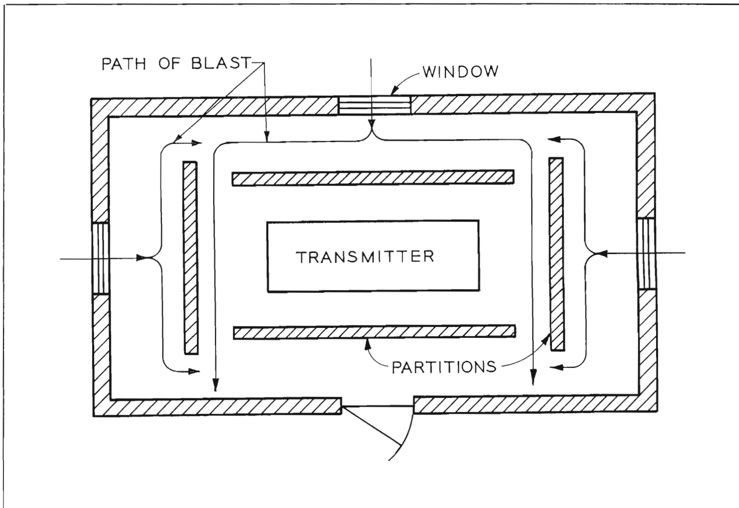
Here is one way of protecting equipment from damage. Leave a free path for the blast to follow and protect equipment with sturdily built partitions.
