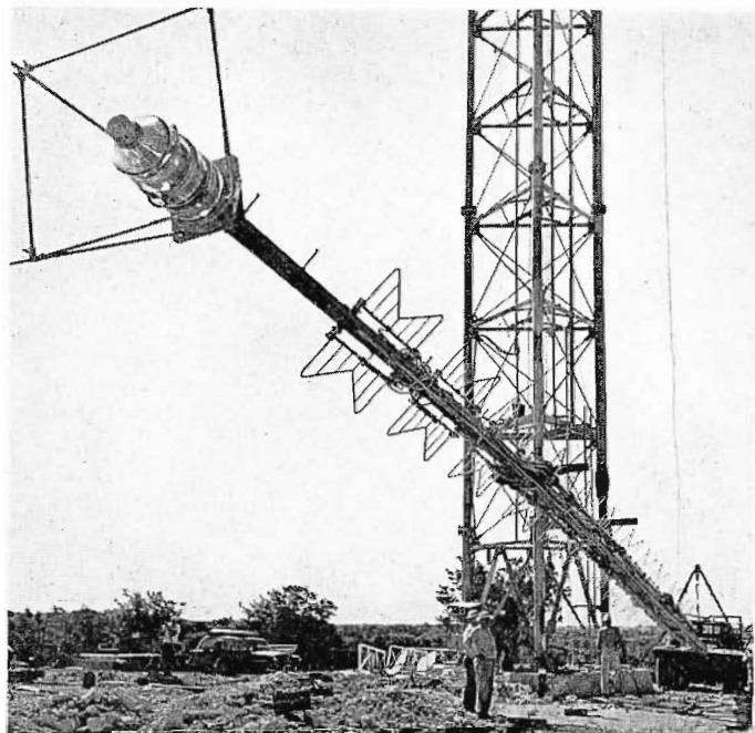
RCA TF-12AH 12-section Superturnstile starts its long journey to the top tower platform. Upper left corner shows detail of beacon and lightning protector.
