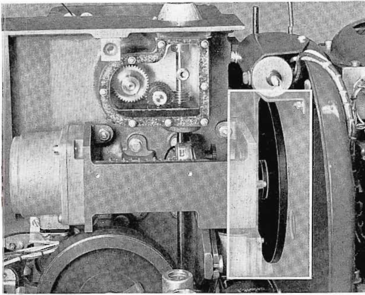
FIG. 8. Light-intensity control mounted in an RCA TP-6CC Projector.
