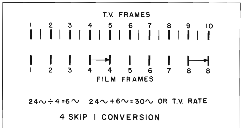
FIG. 5. Relationship of TV frames to film frames in the vidicon method.
