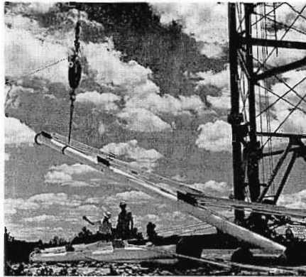
Lower vertical tower members are hoisted into place. They are solid round members 10" in diameter.
