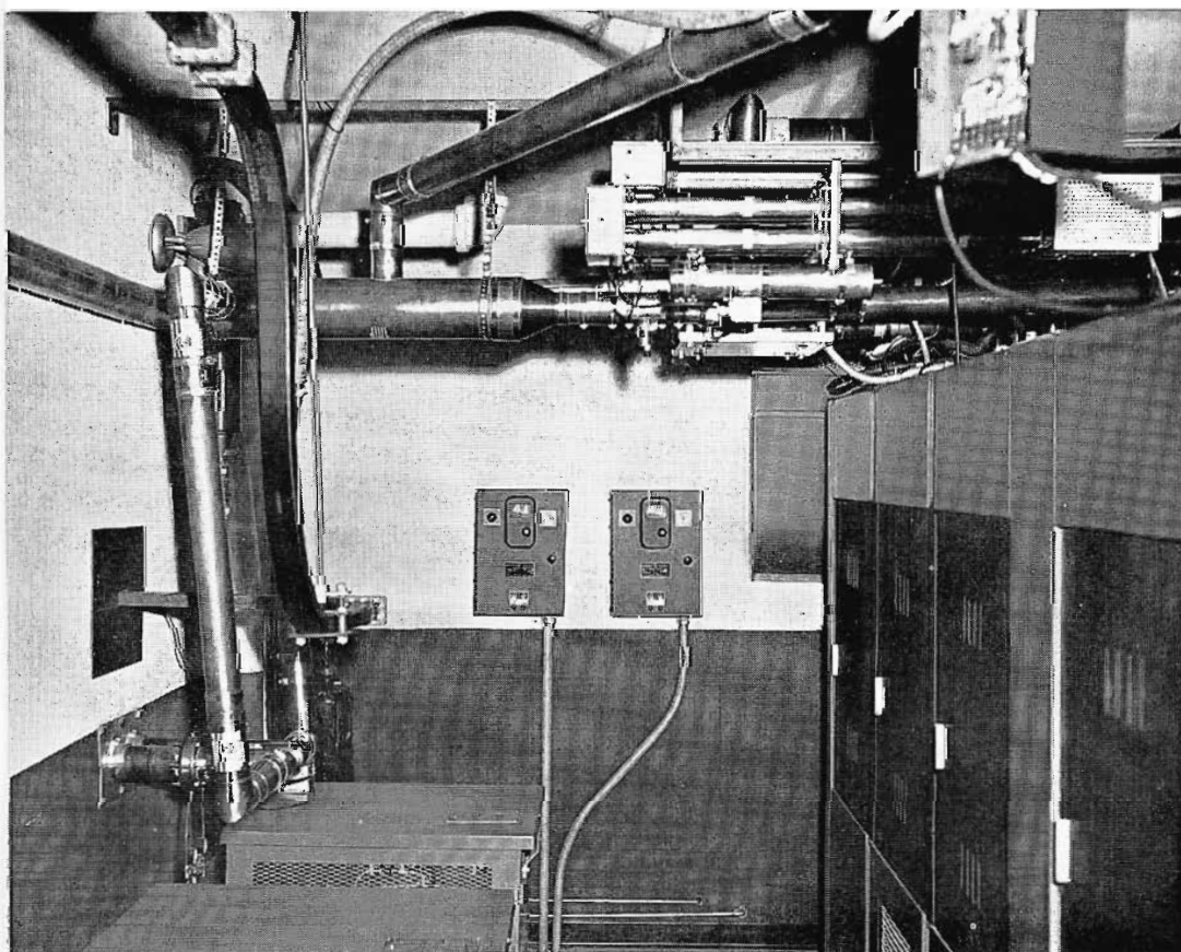
FIG. 11. Rear view of transmitter showing plate transformers, diplexer, coax lines leaving building, filament regulator controls, WM-20 and part of side band filter behind it. Parts of dummy load is visible behind vertical output coax diplexer. Wave guide is AT&T equipment between the antenna and the microwave receiver.
