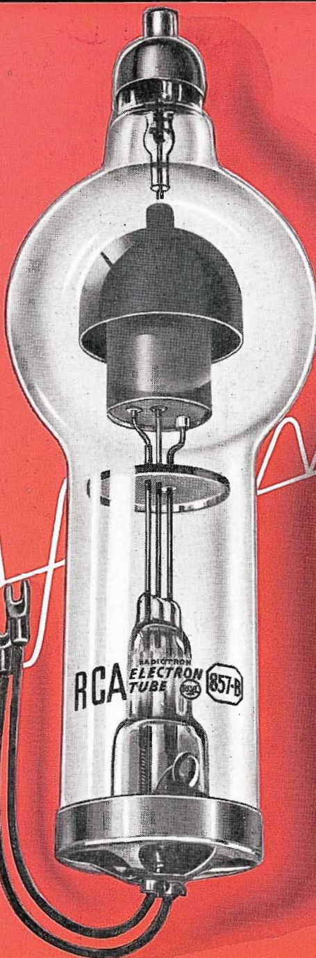
RCA-857B High Power, Mercury-Vapor Rectifier
