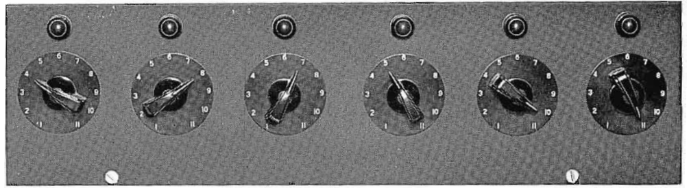
FIG. 6. Mike switch panel for selecting studio mikes.
