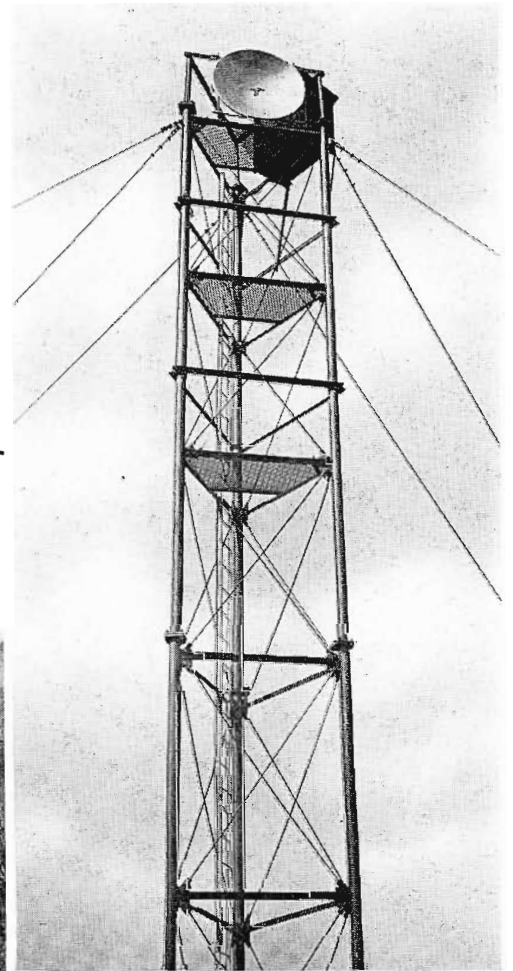
Tower with receiving parabola for pick up of scale model radiated signals.
