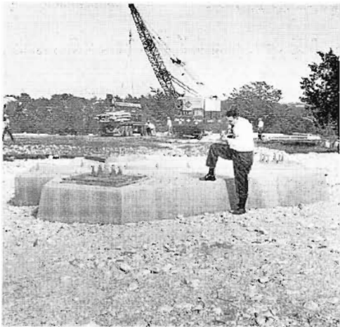
One of many typical guy anchorage piers with steel plates in place.
