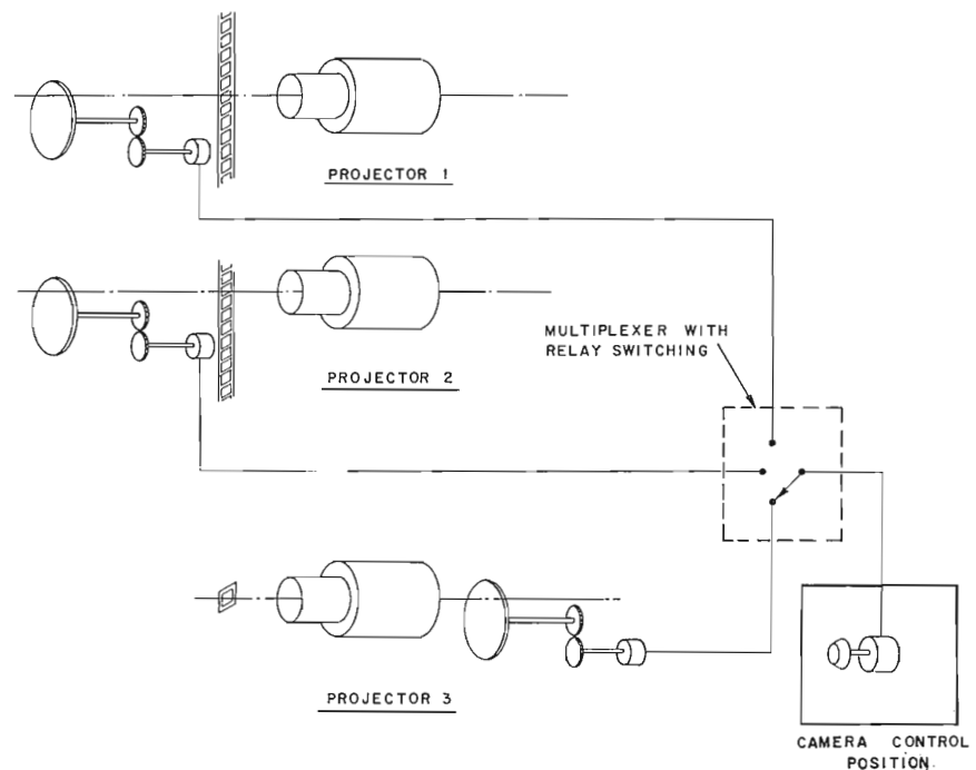
FIG. 10. Multiplexer system for varying light controls.
