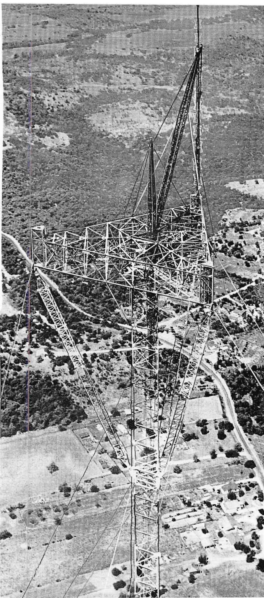
ABOVE—Nearing final construction, this aerial view, taken by the Dallas Morning News, shows RCA 12-Section Superturnstile Antenna of WFAA-TV being mounted.
