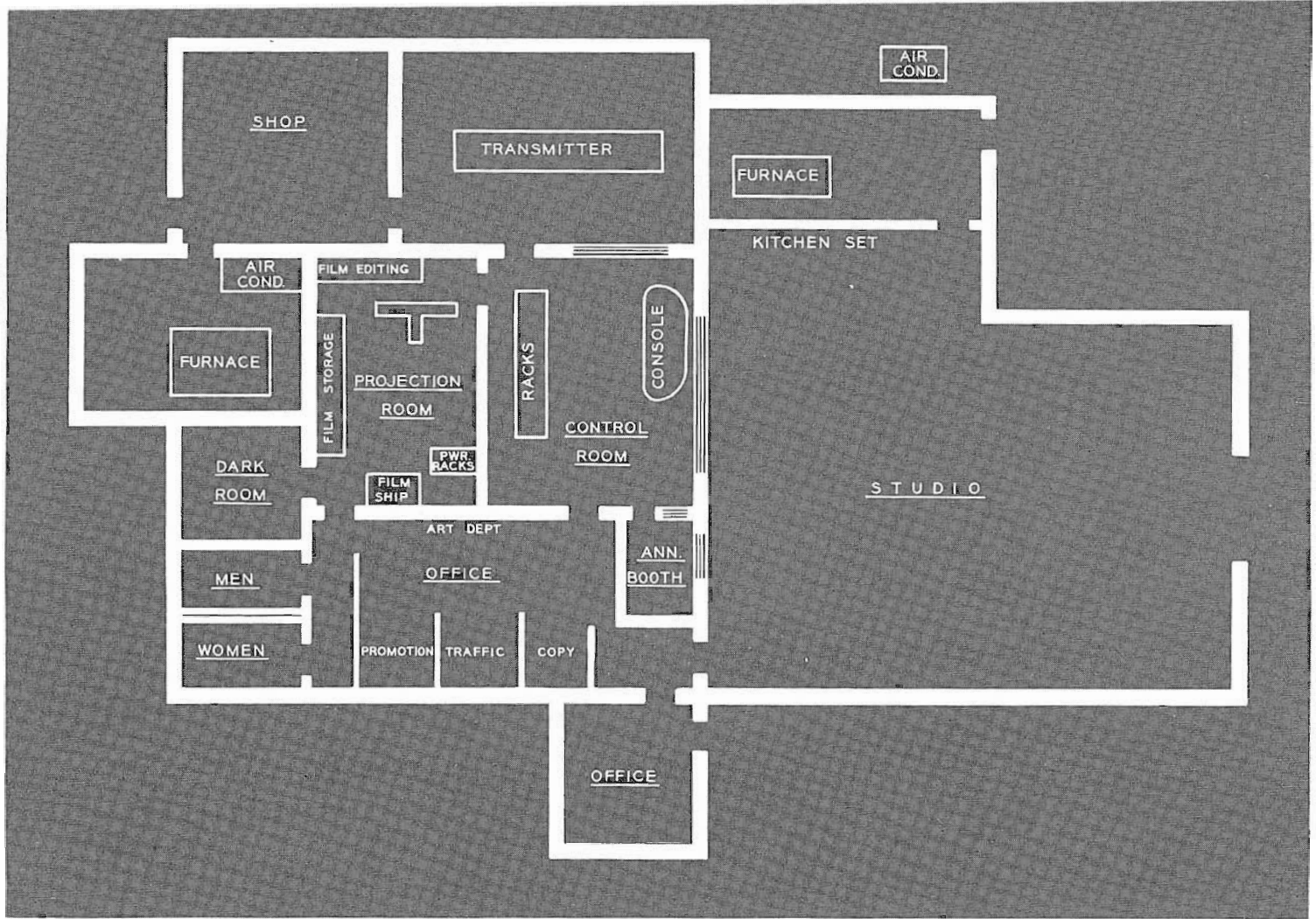
FIG. 4. KROC-TV Floor Plan. Large studio door faces east.
