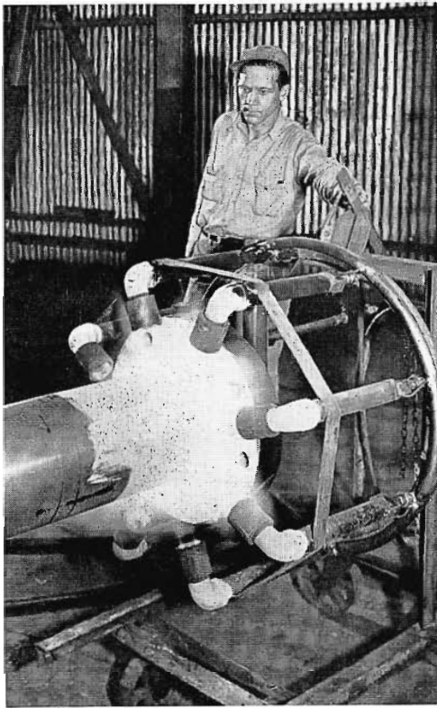
Jig welding of a flange on a round tower leg member by means of a jet welding device.
