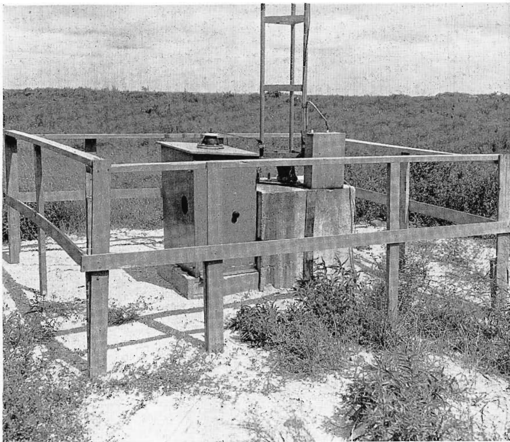
Base of tower with line terminating unit (left) and tower lighting choke (right).
