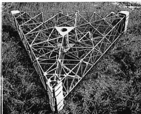
Close-up of scale model tower top upon which model antennas were mounted for testing.
