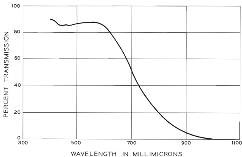
FIG. 5. Transmission characteristics of Pittsburgh heat-absorbing glass Type 2043X 4mm thick.
