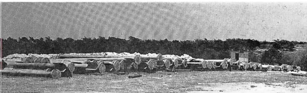
"Battle wagon cannons"? No! . . . solid round vertical tower members up to 10 inches in diameter, 30 feet long and made of Mayari steel—a steel of superior high strength.
