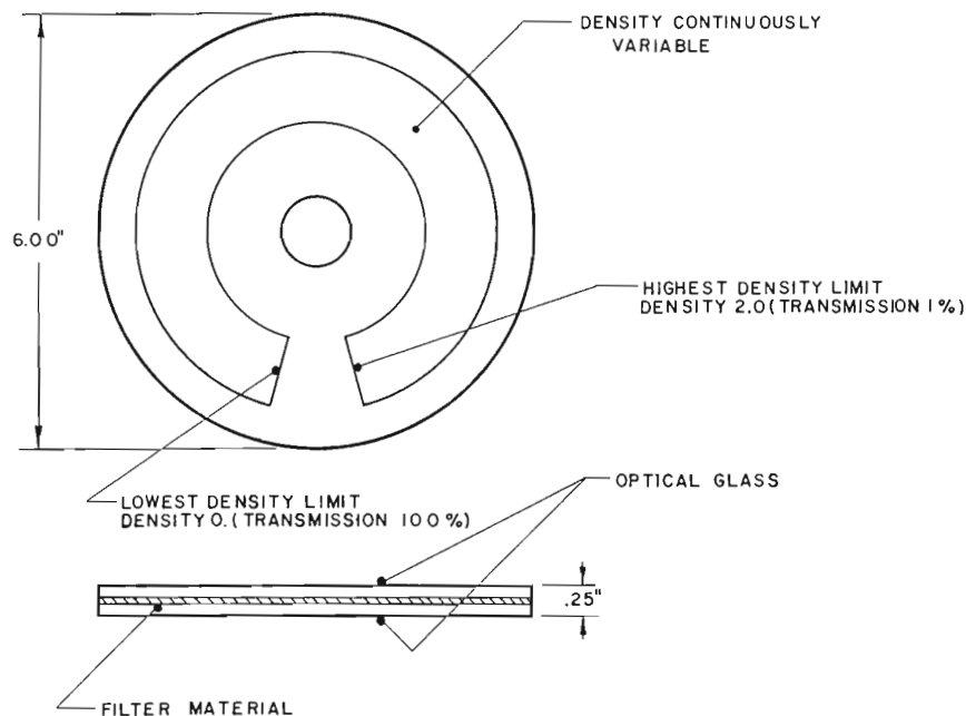
FIG. 2. Outline drawing of the filter wedge used in the light intensity control.
