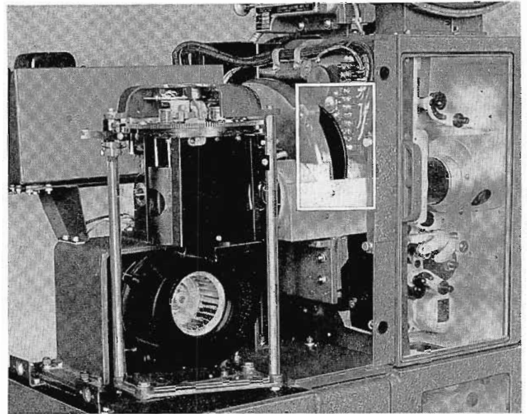
FIG. 9. Light-intensity control mounted in an RCA TP-35CC Projector.
