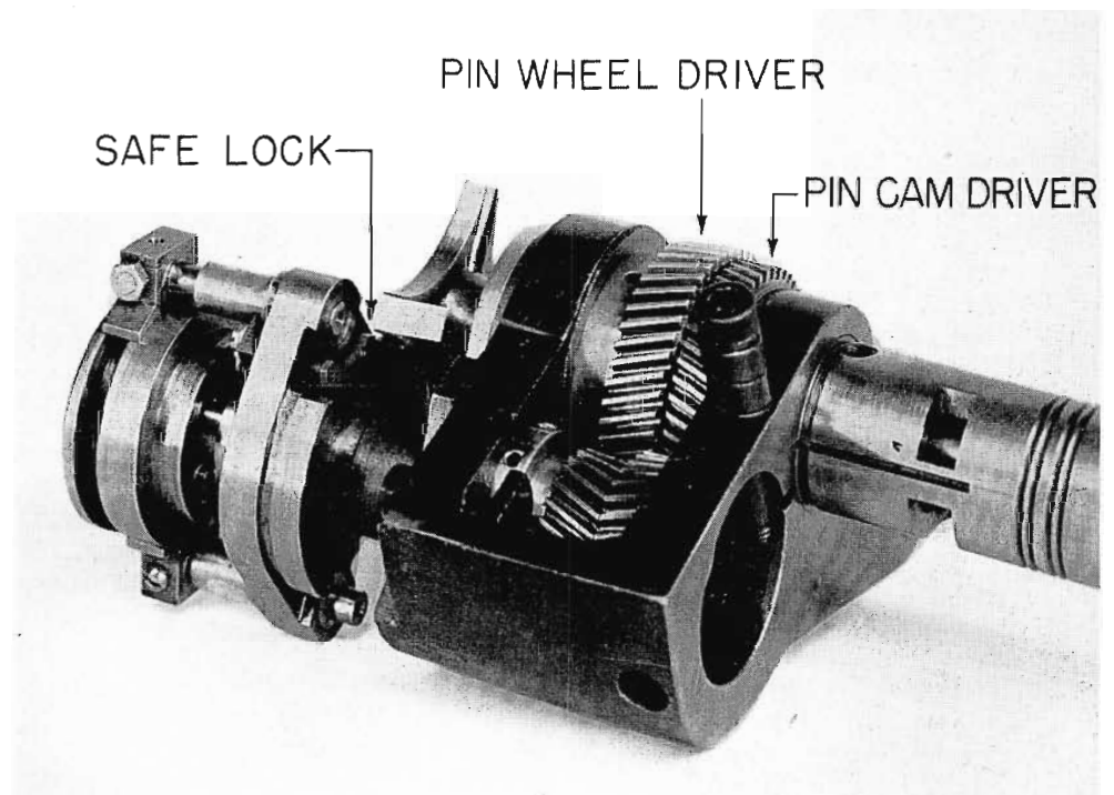
FIG. 7. Close-up of intermittent showing gear mechanism.
