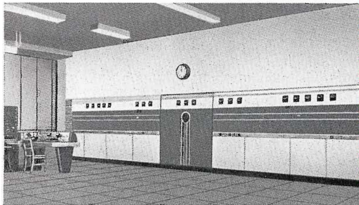
RCA 50-KW Shortwave Transmitter using RCA-857B high-power mercury-vapor rectifiers
