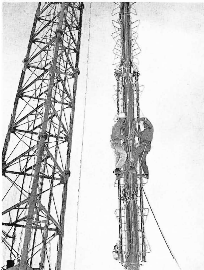
Last minute rigging adjustments are made en route to the top.
