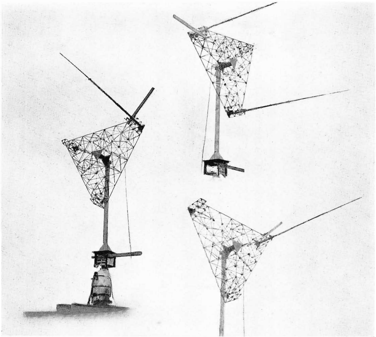
At RCA Moorestown, N. J. Antenna Test Site, scale models of the RCA "Candelabra" Antenna System are conveniently tilted to obtain radiation patterns at various depression angles.
