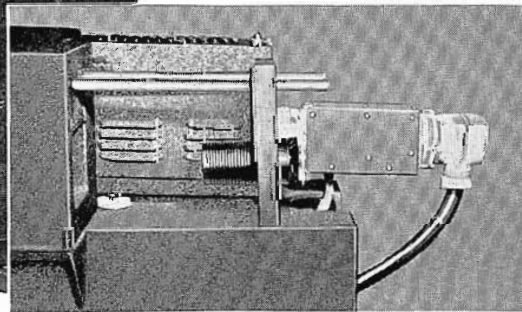
The 9-inch lens is mounted in a block of wood, which slides back and forth for focusing.
