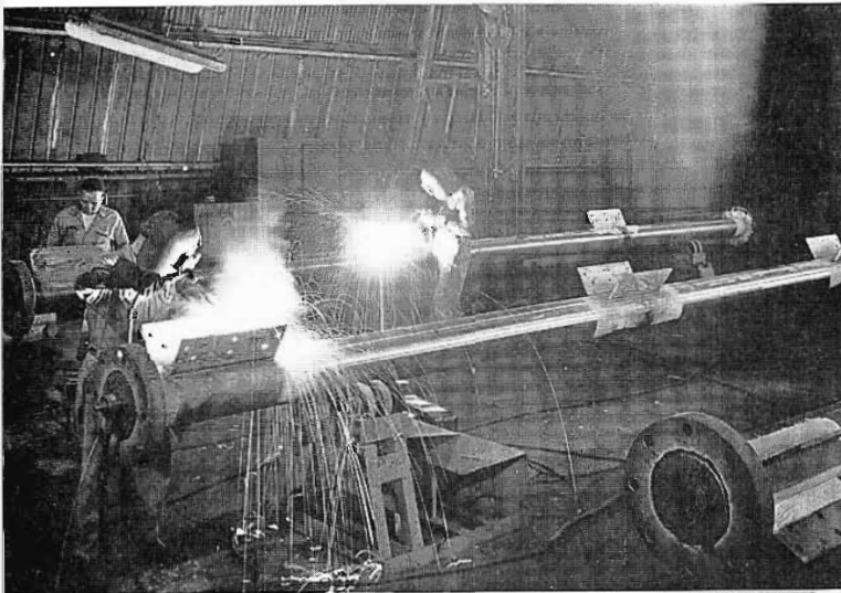
Welding gusset plates into position on round tower leg members. The accurate positioning requirement for these plates is quite evident since tower horizontal and diagonal members will be fastened to them.
