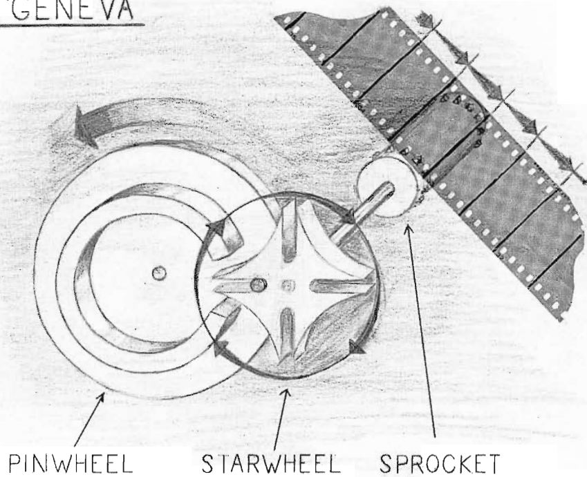
FIG. 4. Simplified diagram of a Geneva mechanism.
