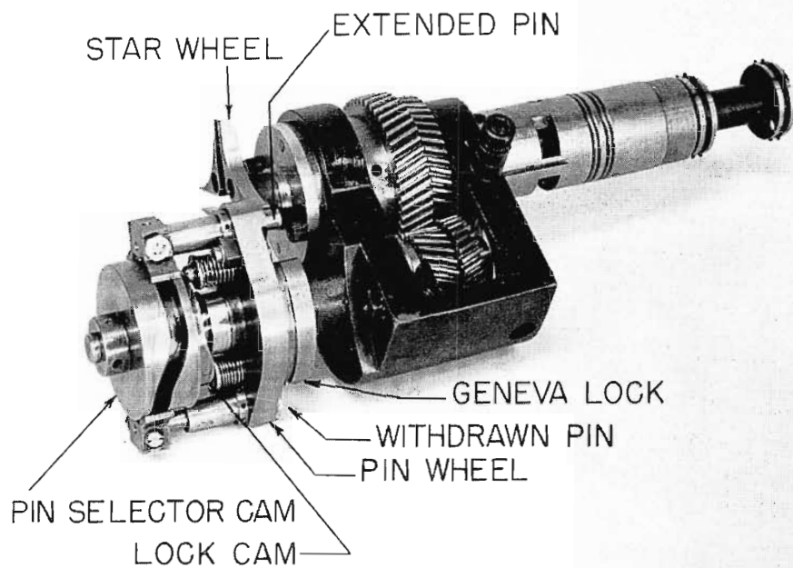
FIG. 6. Overall view of complete intermittent.
