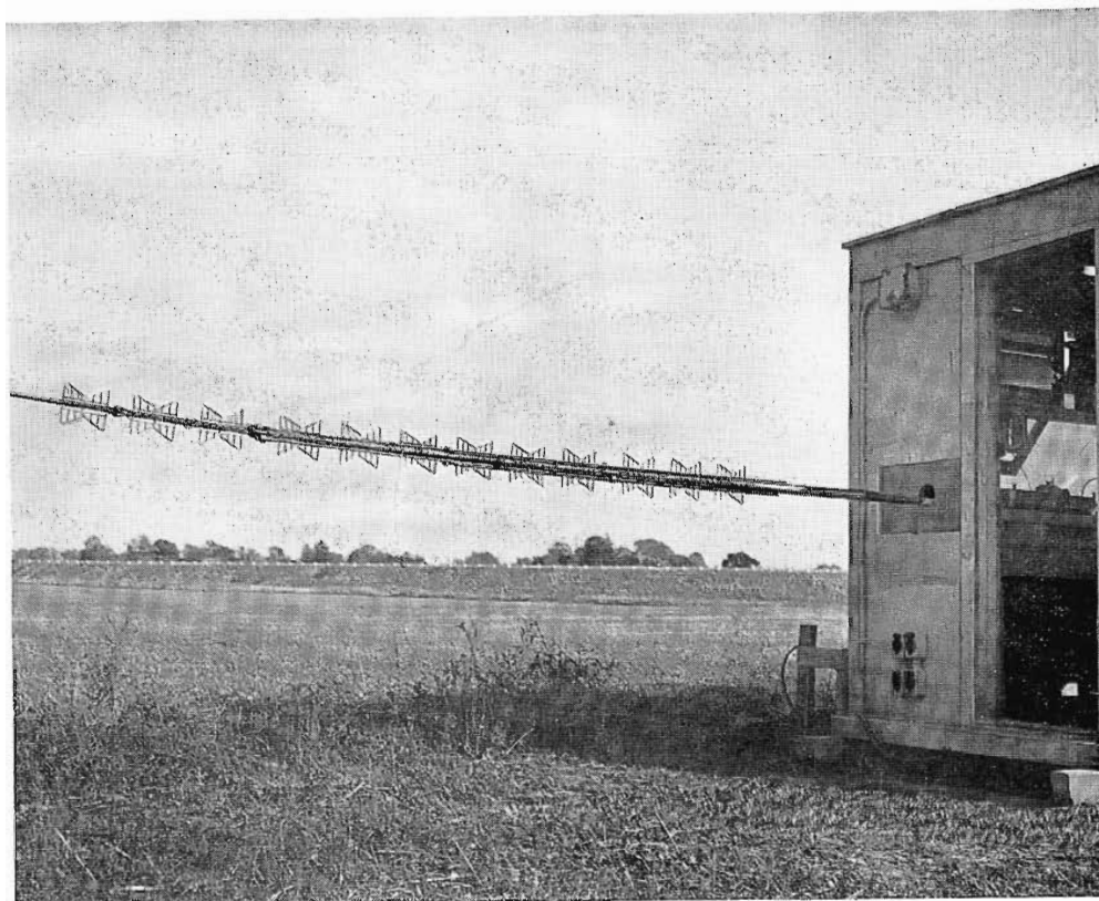
TF-6BM scale model on pattern test set-up.
