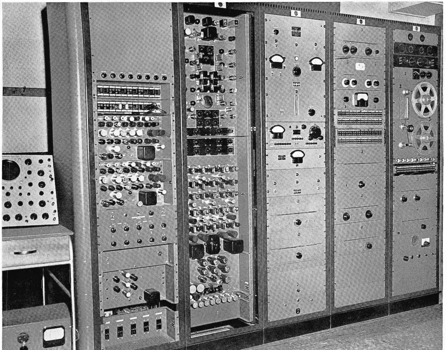
FIG. 7. Equipment racks in KROC-TV control room.
