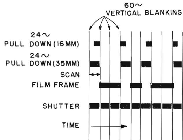
FIG. 2. Relationship between pull-down projectors, shutter, and scanning in prior television practice.
