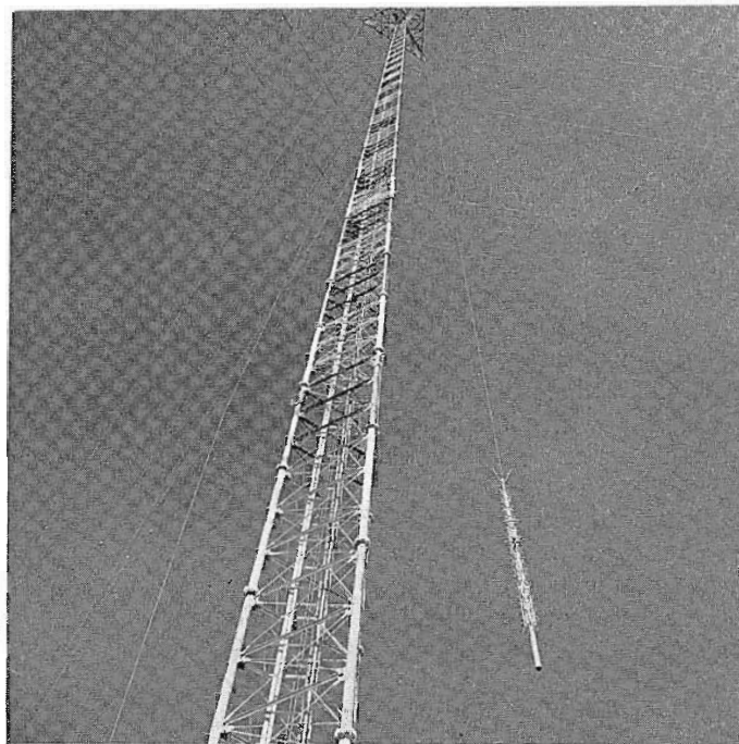
On its way up, the WFAA-TV Channel 8 antenna is carefully guided towards the corner of the triangular tower which it will occupy.
