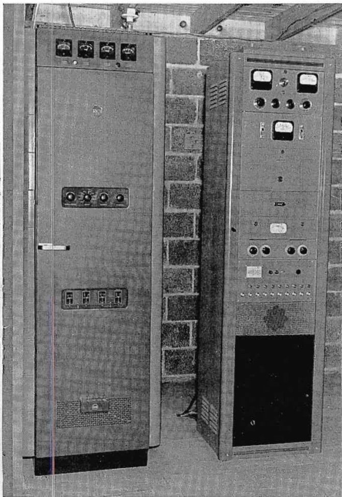
RCA BTA-250M, 250 watt transmitter (left) with RCA BTR-5A remote-control rack (right) constitute the unattended remote-control equipment.
