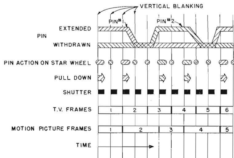
FIG. 3. Relationship between 35mm intermittent, shutter, and television scanning in the RCA vidicon method.
