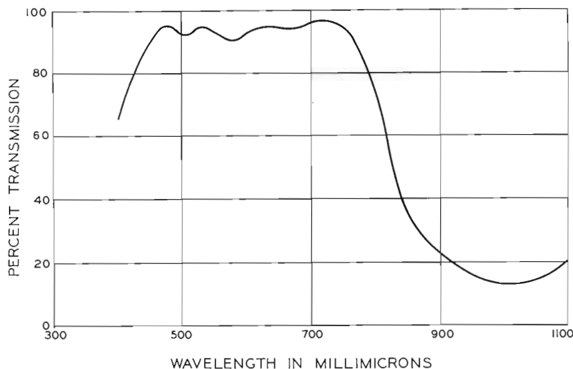
FIG. 4. Spectral transmission curve of Fish-Schurman Type XUR infrared deflector.
