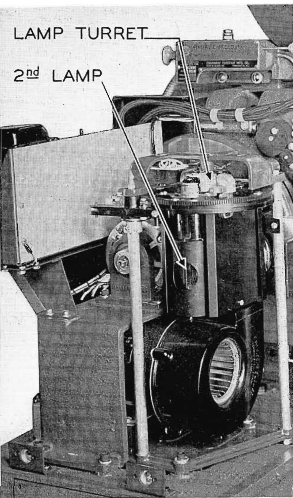
FIG. 8. Close-up of quick-change lamp house.
