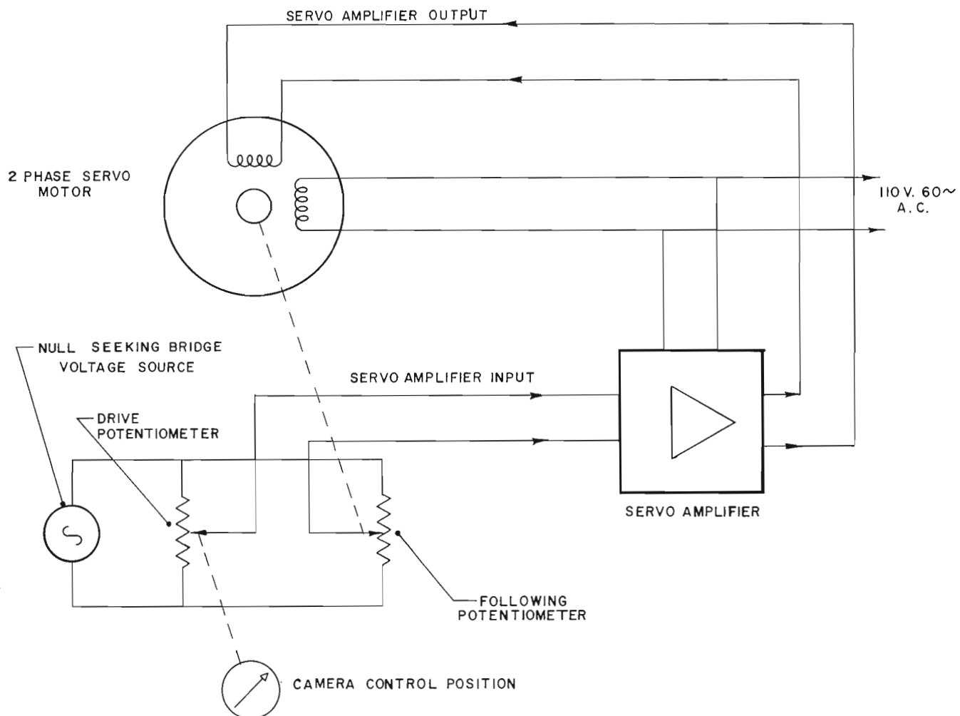
FIG. 3. Bridge circuit which drives the filter wedge.
